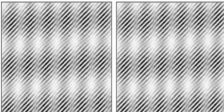
Fig. 5. Reconstruction of an image created with a randomly generated configuration ( N = 7 ). The original image is shown on the left, the reconstruction on the right.
