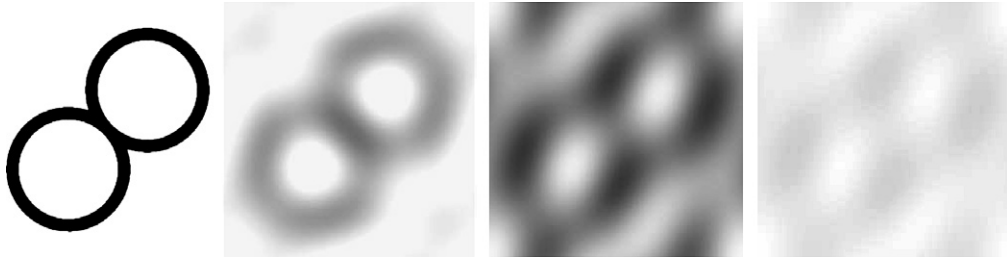
Fig. 13. Here, a different structure was reconstructed. The displayed order is again from left to right: original structure f , best approximation f_d , nonlinear approximations f_s calculated by the coordinate descent method and the Nelder and Mead simplex method.
