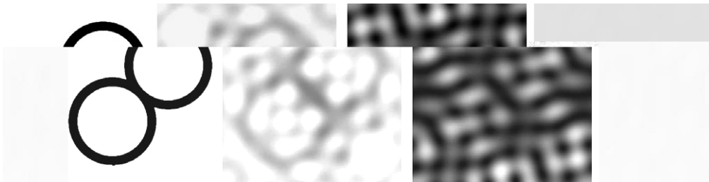
Fig. 17. In this reconstruction with the setup from Fig. 15, a likewise effect occurs as in Fig. 16. The displayed order is again from left to right: f , f_d and f_* calculated with the coordinate descent method and the Nelder and Mead simplex method.
