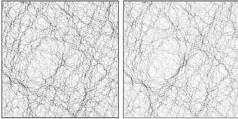
Fig. 6. Reconstruction of an image created with a randomly generated configuration ( N = 101 ).
