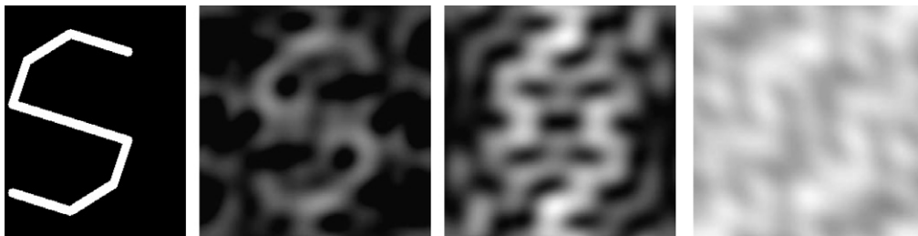
Fig. 18. Here, the beam setup from Fig. 15 is applied to the same image as in Fig. 14. The images are ordered as in all previous figures.
