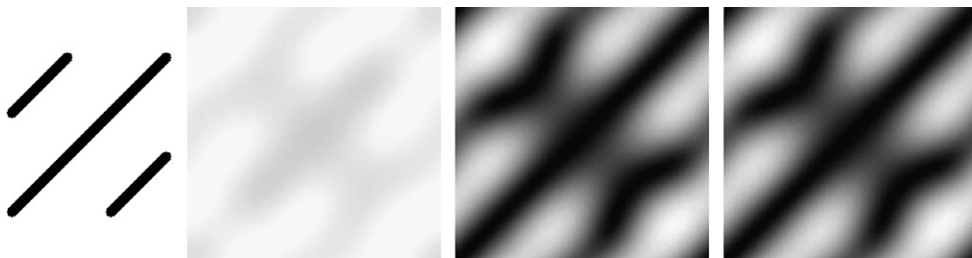
Fig. 12. A simple structure, that was reconstructed by the set \mathcal{K} , as it is sketched in Fig. 11. The two left images show the original structure f (leftmost) and its best approximation f_d from \mathcal{S}_d . On the right, two nonlinear approximations f_* \in \mathcal{S}_N are displayed which were calculated by the Nelder and Mead simplex method (rightmost) and the coordinate descent method.
