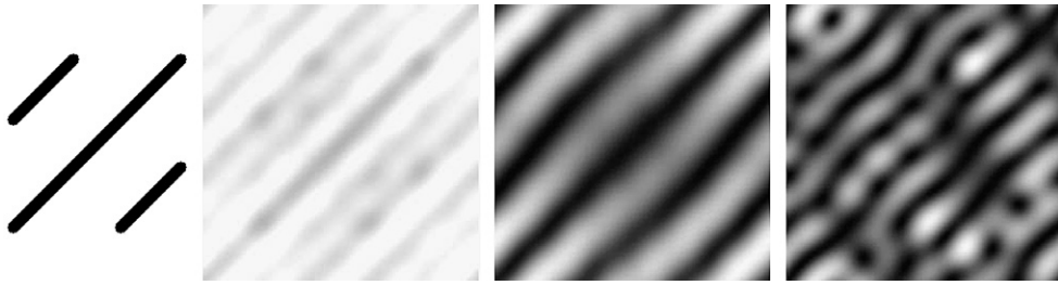
Fig. 16. The original image is the same as in Fig. 12, however this image is reconstructed with the beam setup from Fig. 15. The images show from left to right the original image, the best approximation f_d for this setup and the reconstruction of f_* with the coordinate descent method respectively with the Nelder and Mead simplex method (rightmost).
