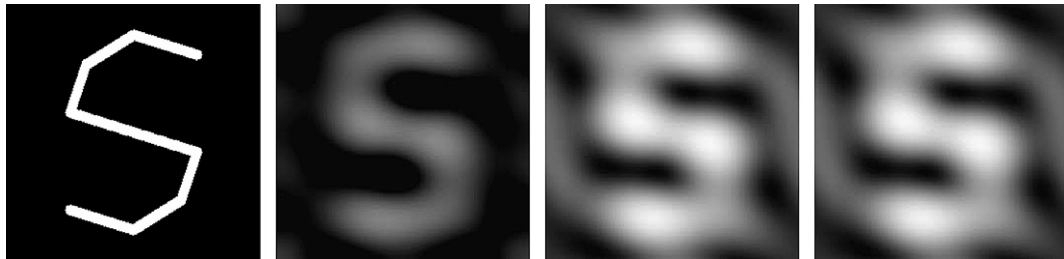
Fig. 14. One more reconstruction with the periodic setup from Fig. 11. The images are ordered as in Figs. 12 and 13.
