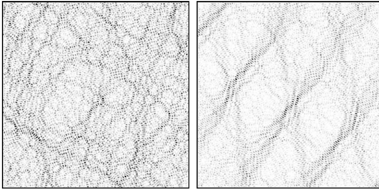
Fig. 9. We display the original image with N = 101 , created from a random configuration of beams, and its reconstruction using an equidistant beam setup with the same number of beams.
