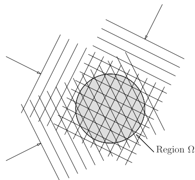
Fig. 1. Schematic view of the interfering light waves. The arrows indicate the directions of propagation of the individual waves, and the parallel lines symbolize the wave fronts. They interfere with each other in the region \Omega , which is drawn as a circle for illustrative purposes. The atomic beam passes this region perpendicular to the paper plane.
